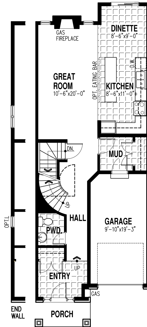
GROUND FLOOR PLAN "B" FINISHED FLOOR AREA = 798 SQ.FT.
