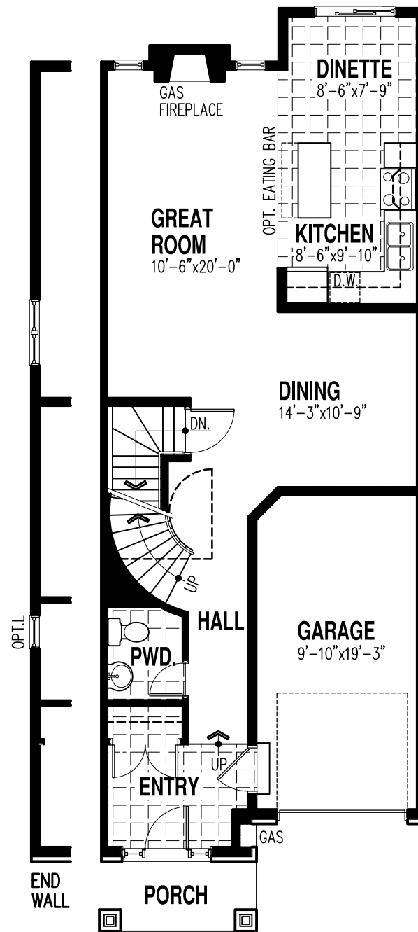
GROUND FLOOR PLAN "A" FINISHED FLOOR AREA = 798 SQ.FT.
