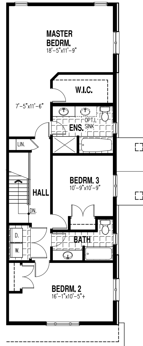
SECOND FLOOR "A" (1,143 Sq Ft. of Finished Floor Area)
