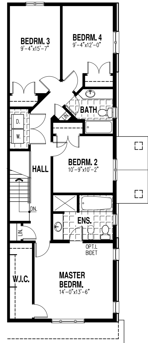
SECOND FLOOR "B" (1,143 Sq Ft. of Finished Floor Area)
