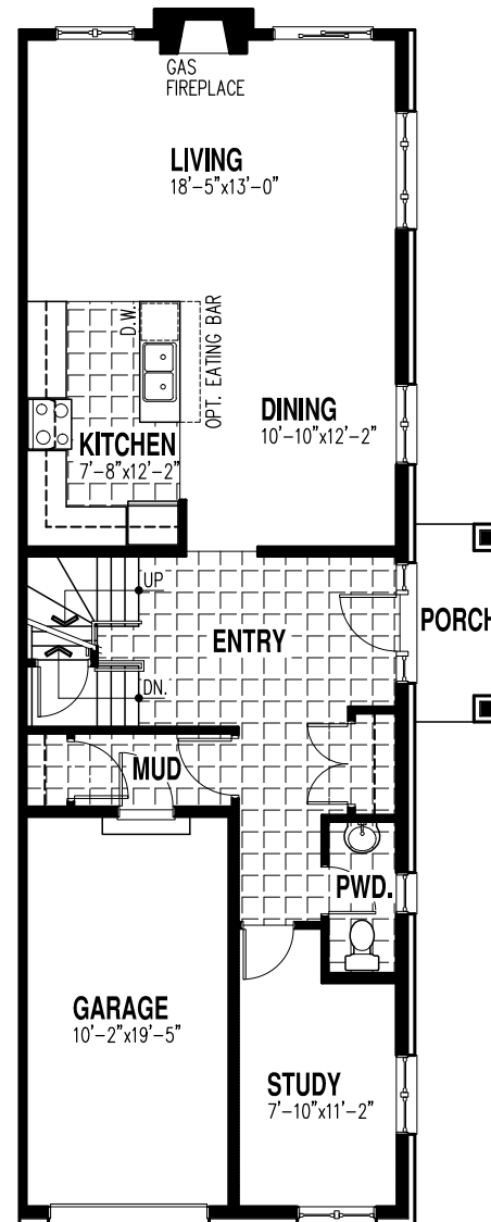
GROUND FLOOR (985 Sq Ft. of Finished Floor Area)
