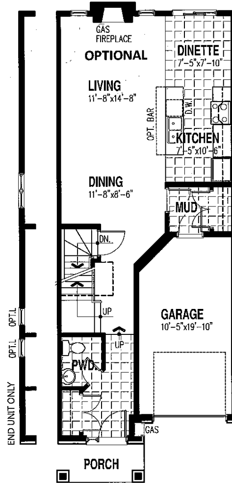
GROUND FLOOR "A" (736 Sq Ft. of Finished Floor Area)
