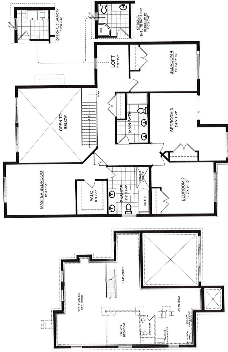
BASEMENT FLOOR
