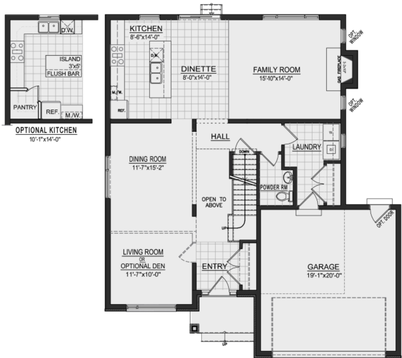
FIRST FLOOR
