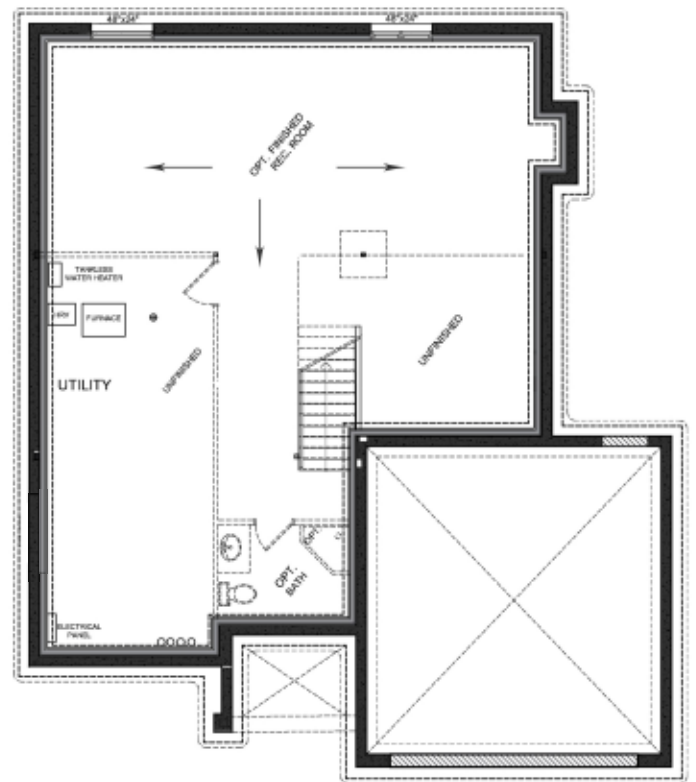
BASEMENT FLOOR
