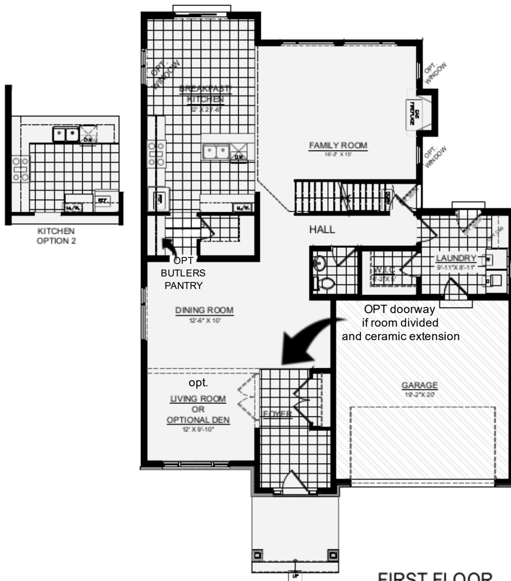
FIRST FLOOR
