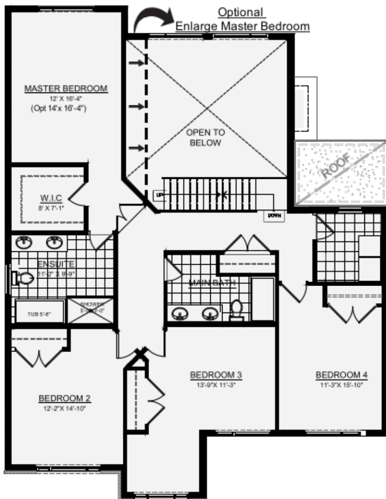
SECOND FLOOR
