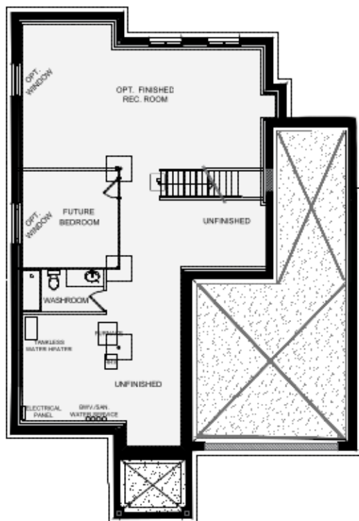
BASEMENT FLOOR
