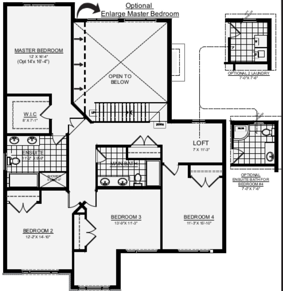
SECOND FLOOR
