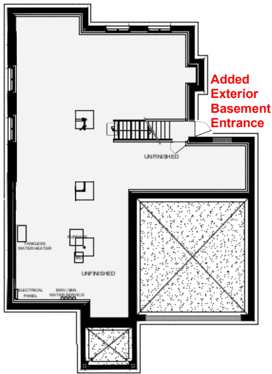
BASEMENT FLOOR
